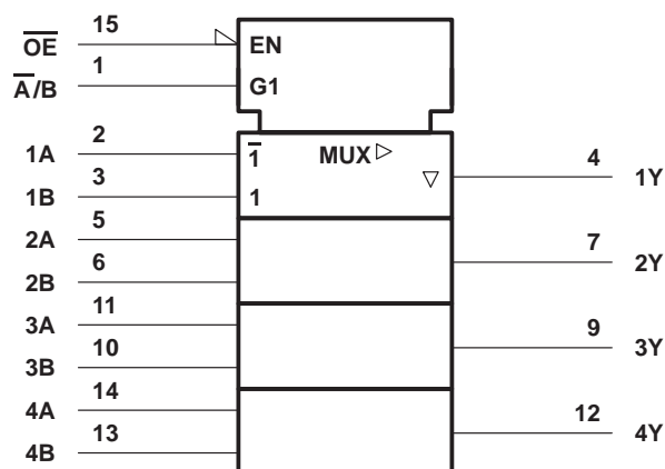
SN54ALS257, SN74ALS257A, SN74AS257
