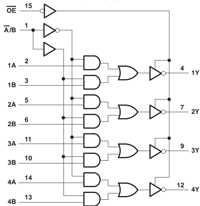
SN54ALS258, SN74ALS258A, SN74AS258
