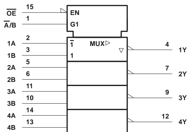
SN54ALS258, SN74ALS258A, SN74AS258
