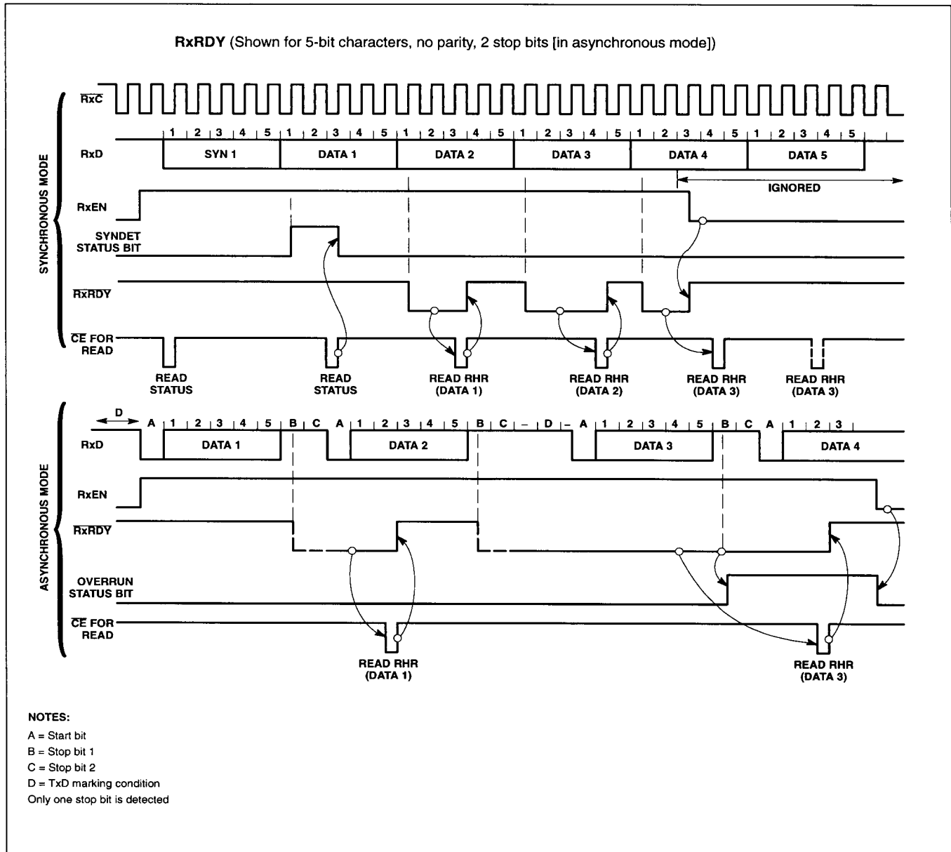
TIMING DIAGRAMS (Continued)
