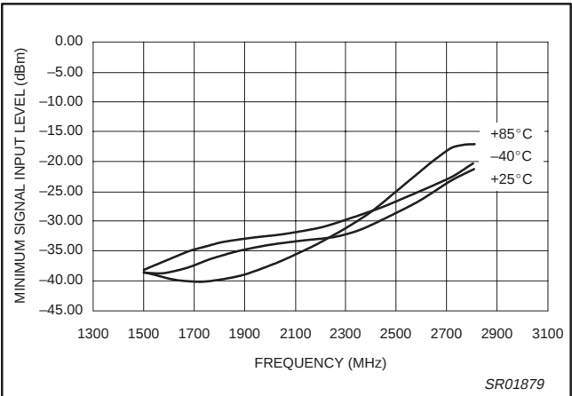
Figure 26. Main Divider Input Sensitivity vs. Frequency and Temperature ( V_{DD} = 3.00 V )
