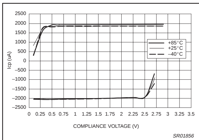
Figure 10. PHI Charge Pump Output vs. Temperature (CP = 01; V_{DD} = 3.0 V; I_{SET} = 165.33 \mu A)
