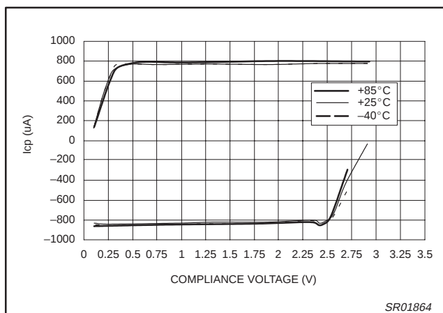
Figure 18. PHP-SU Charge Pump Output vs. Temperature (CP = 01; V_{DD} = 3.0 V; I_{SET} = 165.33 μA)
