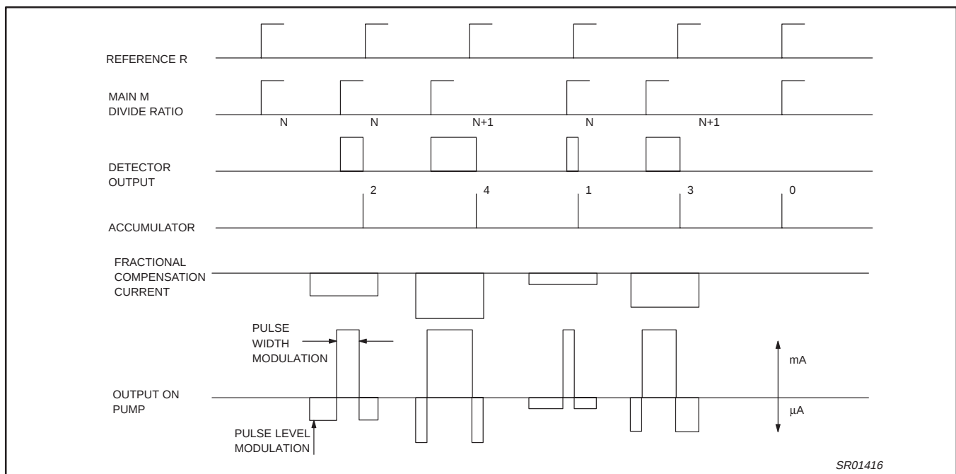
Figure 6. Waveforms for NF = 2 Modulo 5 \rightarrow fraction = 2/5
