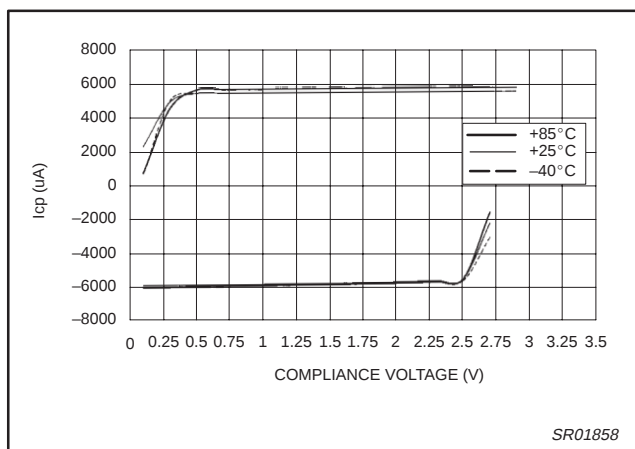
Figure 12. PHI Charge Pump Output vs. Temperature (CP = 00; V_{DD} = 3.0 V; I_{SET} = 165.33 \mu A)
