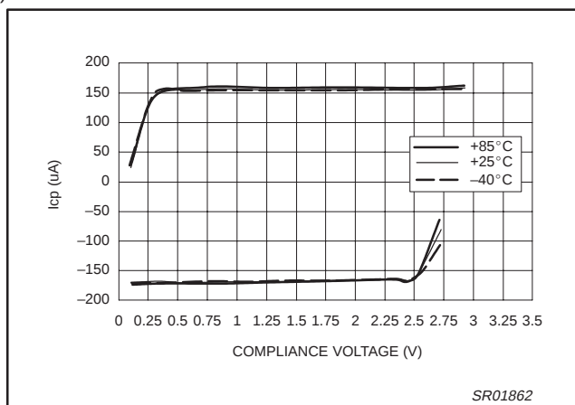
Figure 16. PHP Charge Pump Output vs. Temperature (CP = 11; V_{DD} = 3.0 V; I_{SET} = 165.33 μA)
