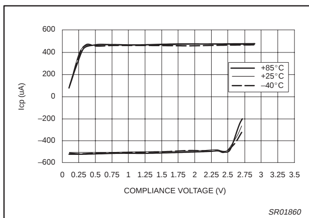
Figure 14. PHP Charge Pump Output vs. Temperature (CP = 10; V_{DD} = 3.0 V; I_{SET} = 165.33 \mu A)
