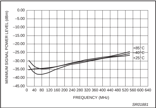
Figure 28. Auxiliary Divider Input Sensitivity vs. Frequency and Temperature (Supply = 3.00 V)
