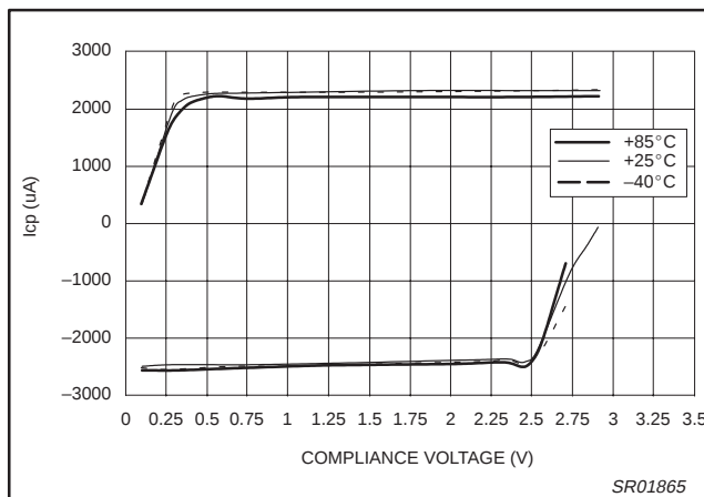
Figure 20. PHP-SU Charge Pump Output vs. Temperature (CP = 00; V_{DD} = 3.0 V; I_{SET} = 165.33 μA)
