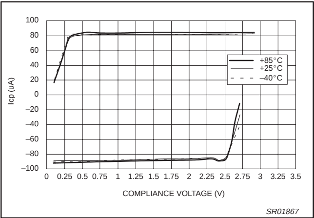
Figure 22. PHA Charge Pump Output vs. Temperature (CP = 11; V_{DD} = 3.0 V ; I_{SET} = 165.33 \mu A )
