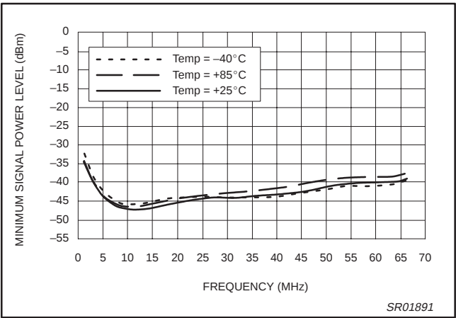
Figure 30. Reference Divider Input Sensitivity vs. Frequency and Temperature (VDD = 3.00 V)
