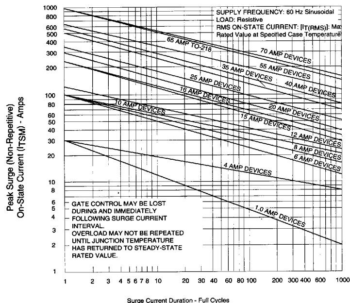
Figure 10—Peak Surge Current vs Surge Current Duration
