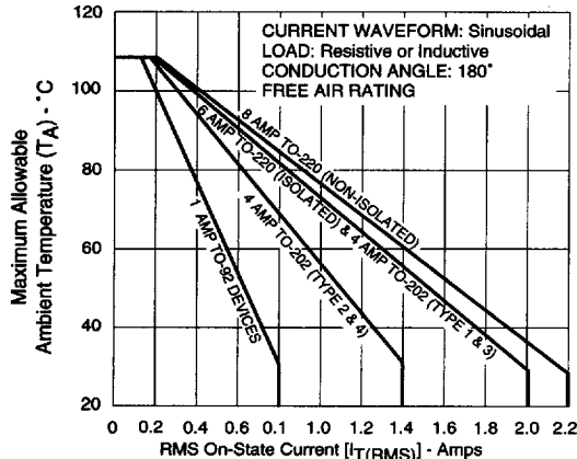
Figure 1A—Maximum Allowable Ambient Temperature vs RMS On-State Current
