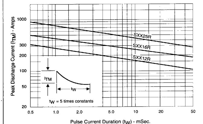
Figure 2A — Peak Capacitor Discharge Current
