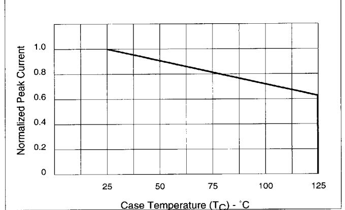
Figure 2B — Peak Capacitor Discharge Current Derating
