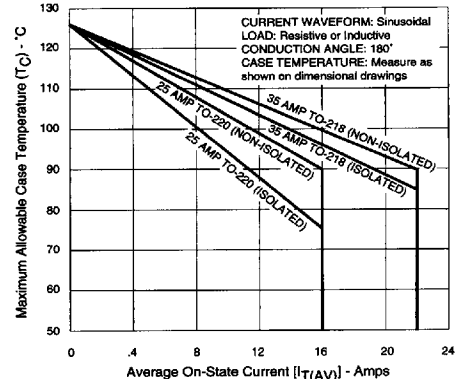
Figure 4D—Maximum Allowable Case Temperature vs Average On-State Current
