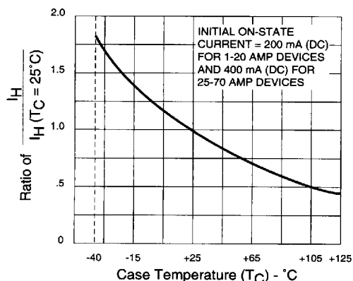
Figure 5—Normalized DC Holding Current vs Case Temperature
