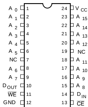
SOJ (14) Top View
