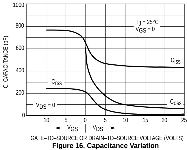
Figure 16. Capacitance Variation
