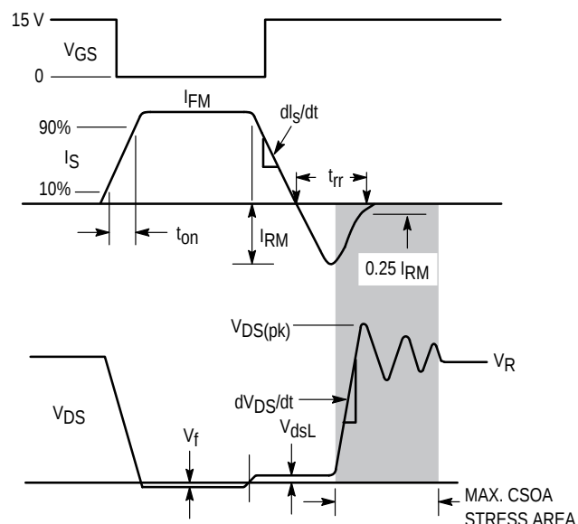
Figure 11. Commutating Waveforms
