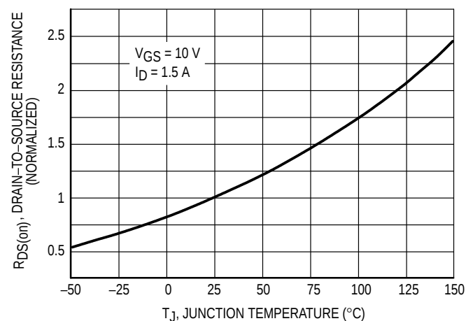
Figure 6. On-Resistance versus Temperature
