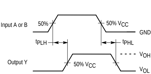
Figure 3. Switching Waveforms
