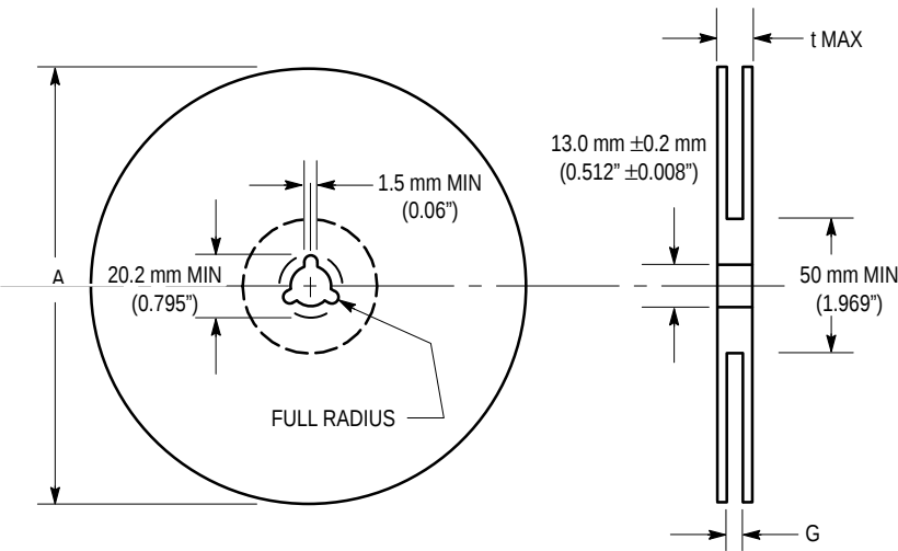
Figure 6. Reel Dimensions
