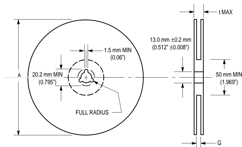
Figure 6. Reel Dimensions
