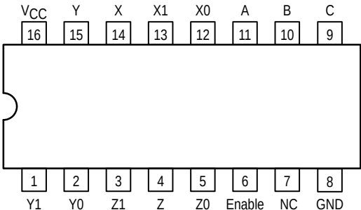
Pinout: MC74LVX8053 (Top View)
