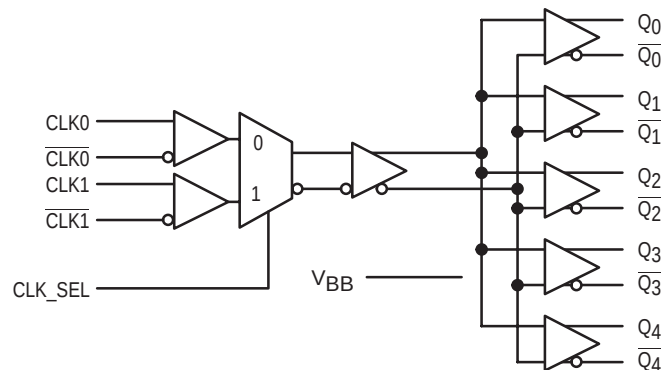
Figure 2. Logic Symbol
