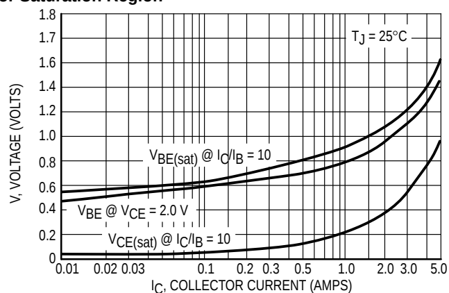
Figure 4. "On" Voltage
