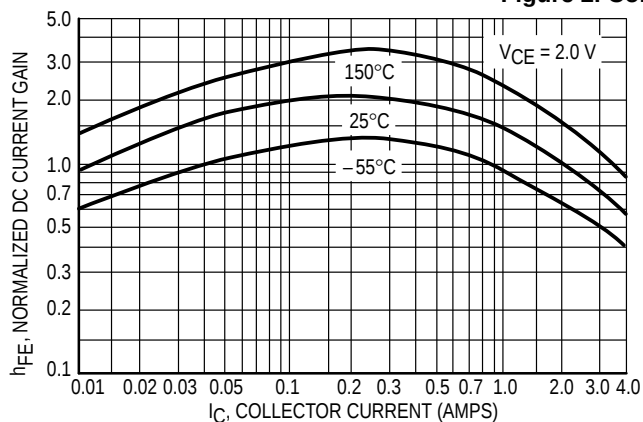
Figure 3. Normalized DC Current Gain
