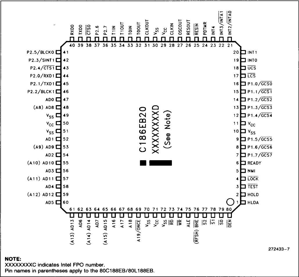
Figure 6. SQFP Package
