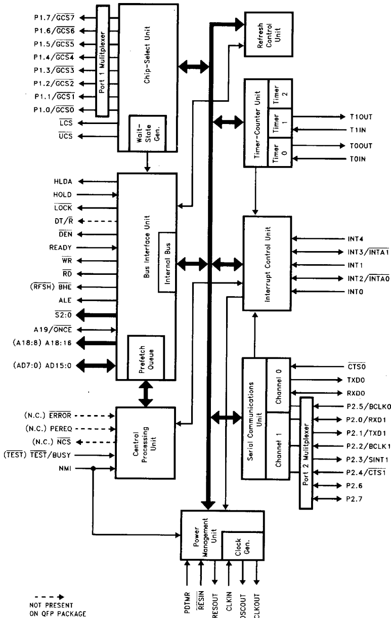
Figure 1. 80C186EB/80C188EB Block Diagram
