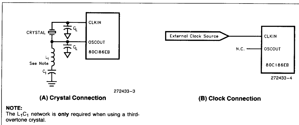
Figure 2. Clock Configurations
