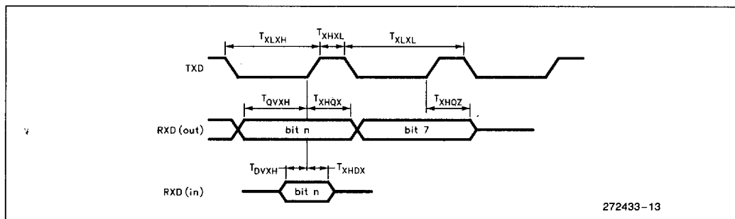
Figure 12. Serial Port Mode 0 Waveform
