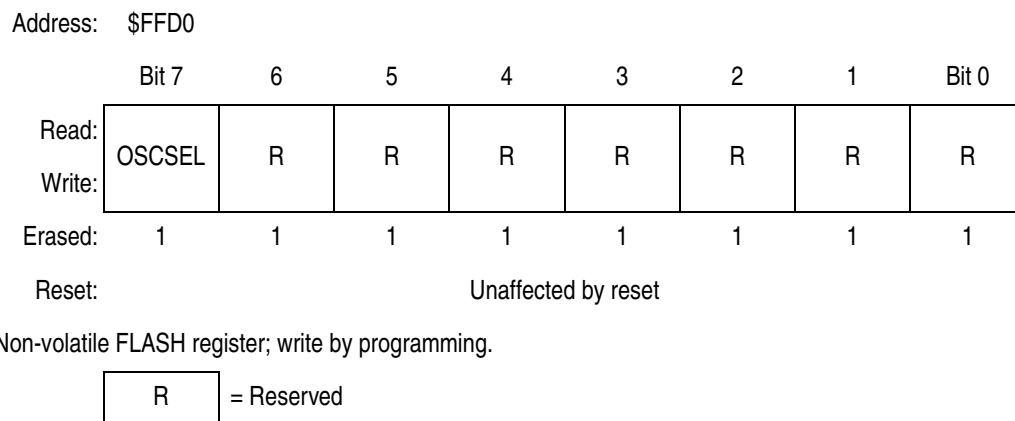
Figure 5-4. Mask Option Register (MOR)
