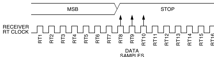
Figure 11-7. Slow Data
