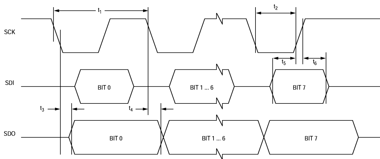
Figure 14-1. SIOPTiming Diagram
