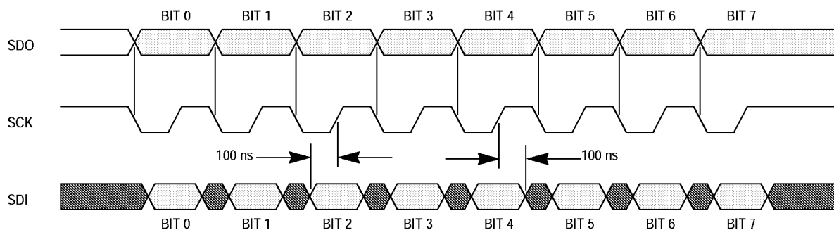
Figure 7-2. SIOP Timing Diagram
