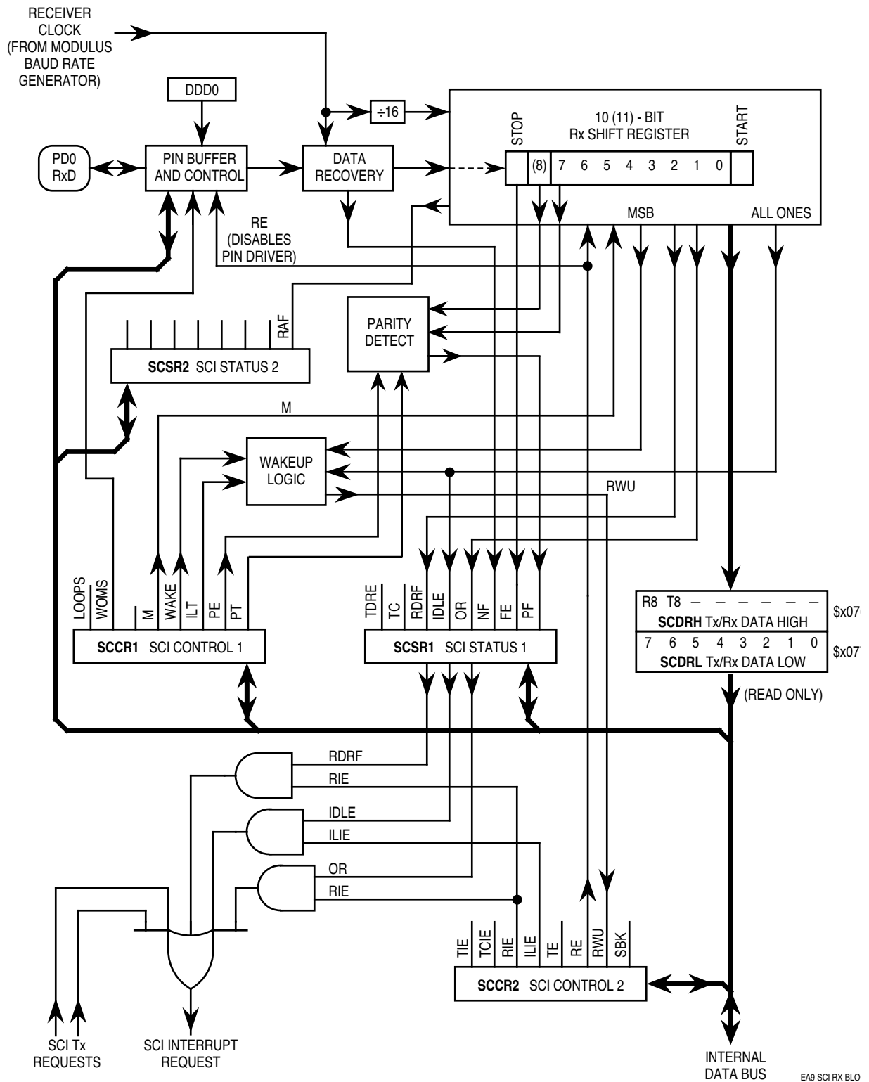
Figure 13 SCI Receiver Block Diagram
