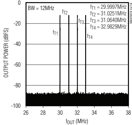
FOUR-TONE POWER RATIO PLOT ( f_{CLK} = 150MHz )
