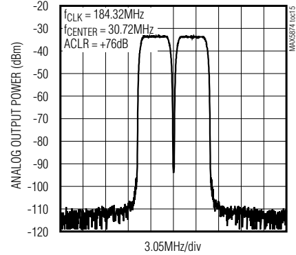
ACLR FOR W-CDMA MODULATION TWO CARRIER
