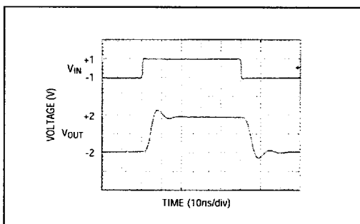
Figure 4a. Large-Signal Pulse Response with C_L = 100\text{pF} and R_{ISO} = 5.1\Omega
