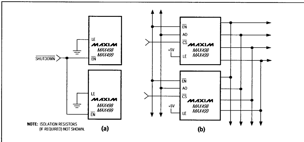
Figure 8. (a) Simultaneous Shutdown of all MAX498/MAX499s; (b) Enable (EN) Register Latched by CS
