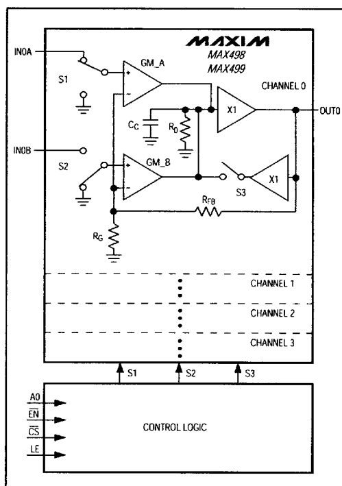
Figure 2. Block Diagram
