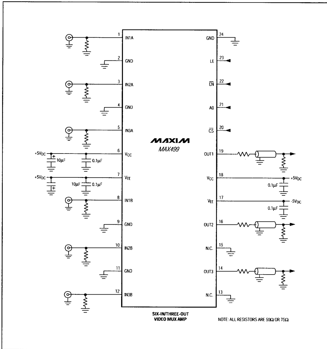
Figure 1b. MAX499 Typical Application Circuit
