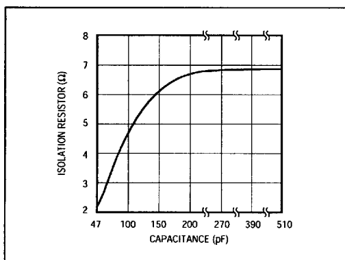
Figure 5. Isolation Resistor vs. Capacitive Load
