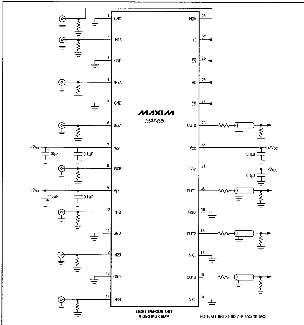
Figure 1a. MAX498 Typical Application Circuit
