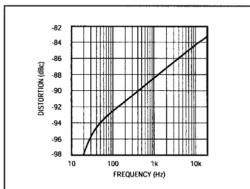
Figure 6. Total Harmonic Distortion (Audio) vs. Frequency
