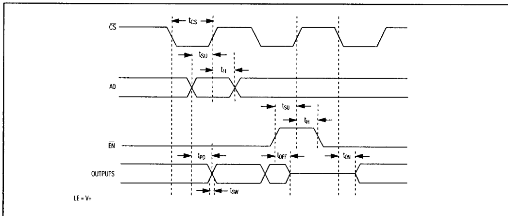
Figure 7. Logic Timing Diagram
