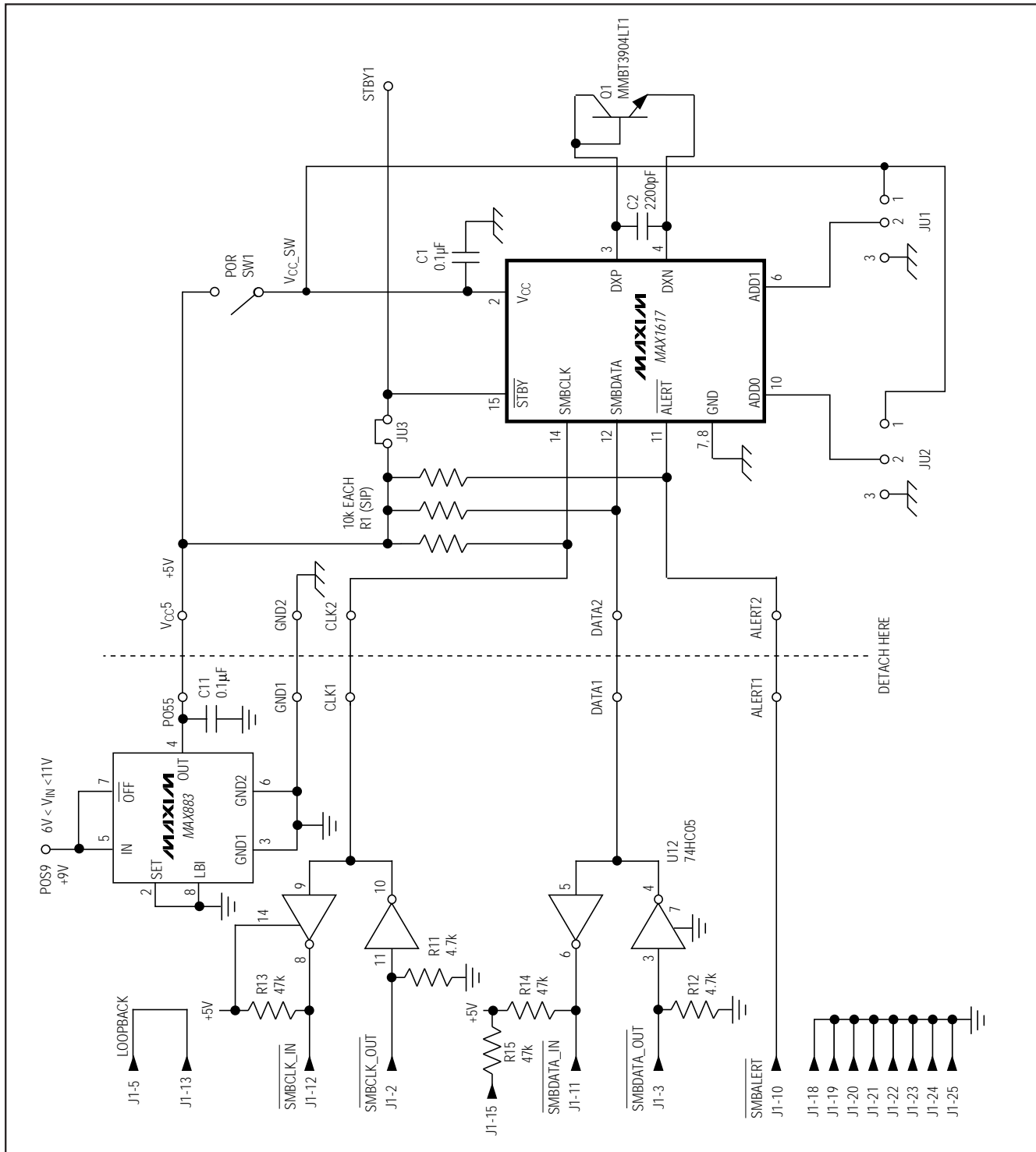
Figure 1. MAX1617 EV Kit Schematic
