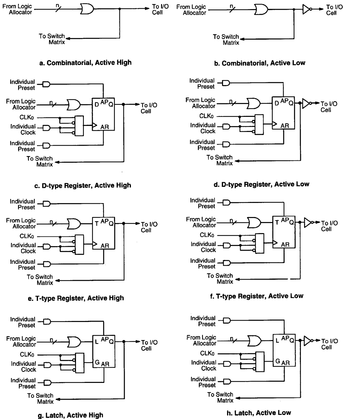
Figure 4. Output Macrocell Configurations
