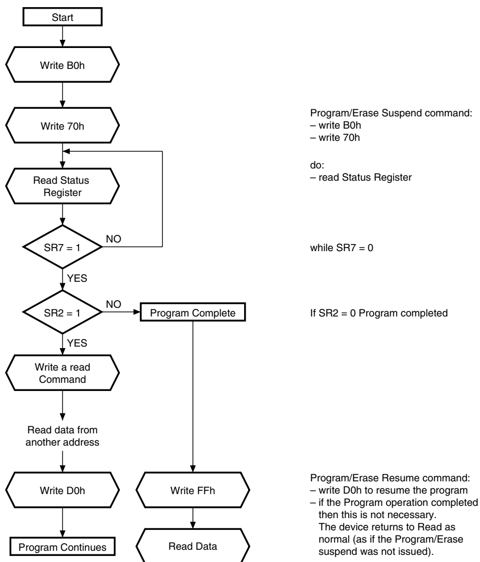
Figure 21. Program Suspend and Resume Flowchart and Pseudo Code
