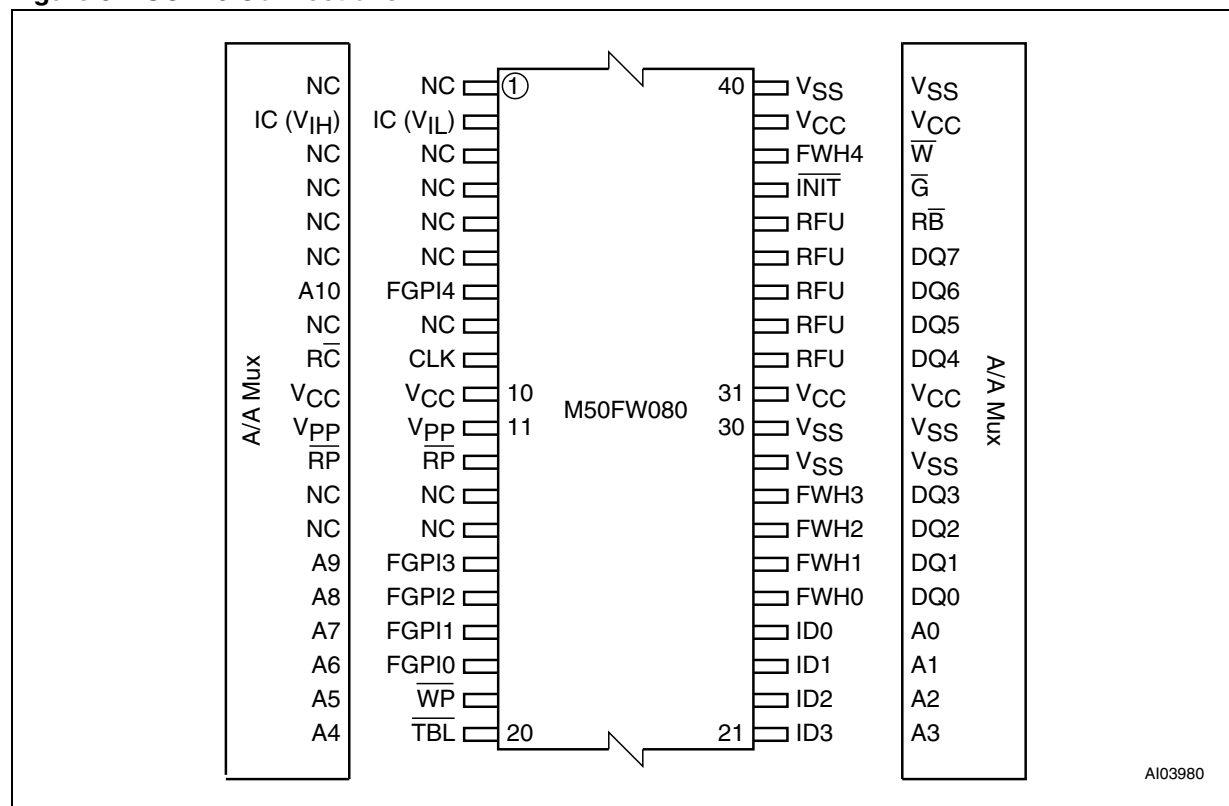
Figure 6. TSOP40 Connections
