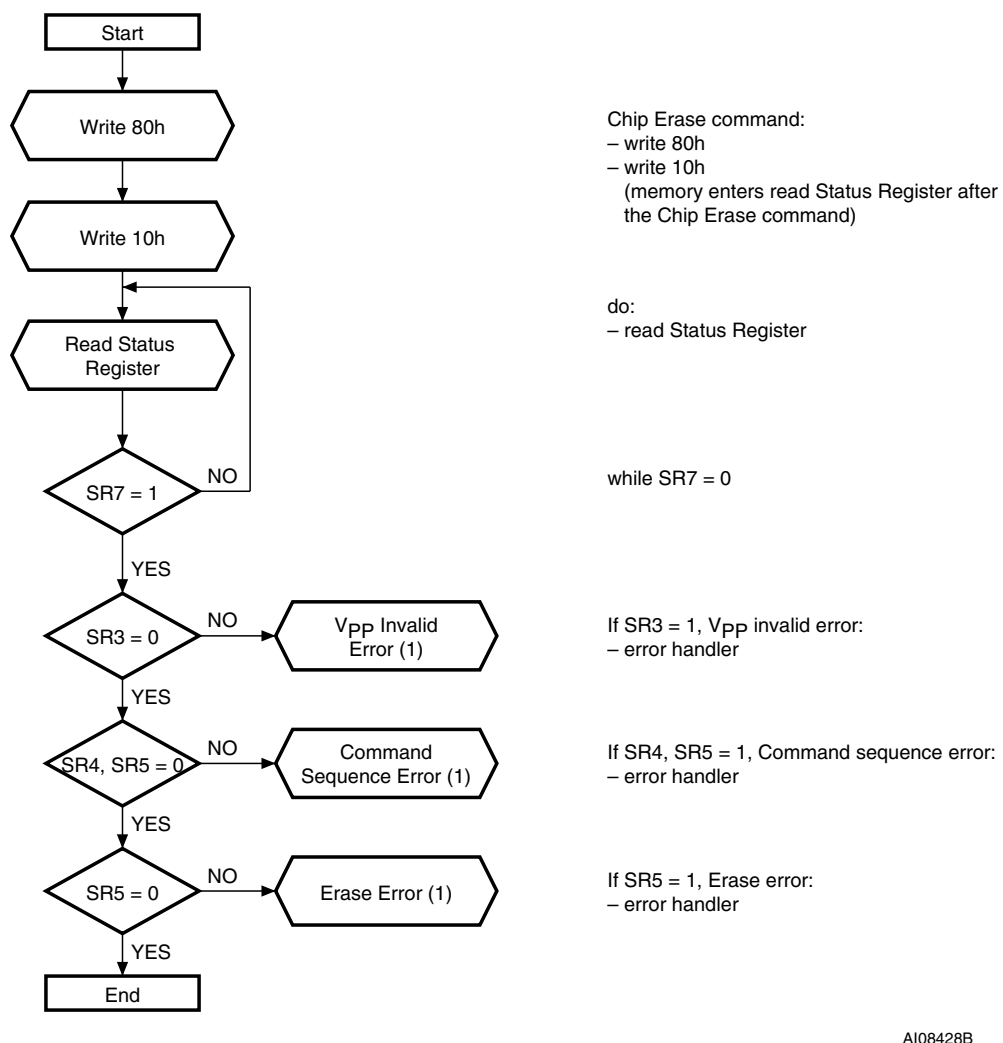
Figure 22. Chip Erase Flowchart and Pseudo Code (A/A Mux Interface Only)
