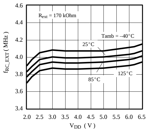
Figure 93. External RC frequency vs. V_{DD}
