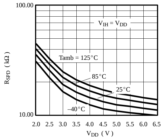
Figure 102. Strong pull-down resistor vs. V_{DD}
