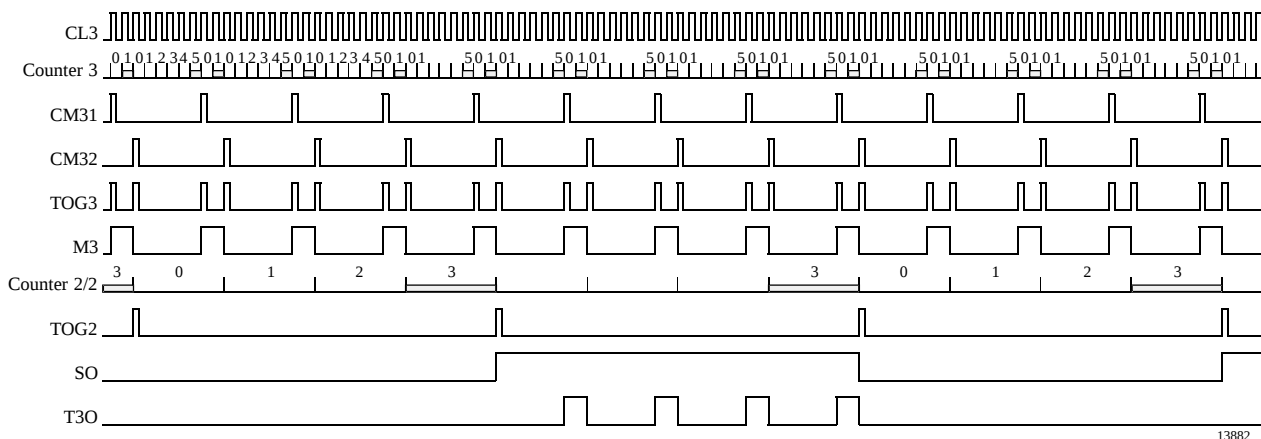
Figure 84. Burst modulation 2
