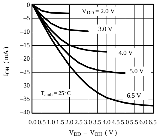
Figure 100. Output high current vs. V_{DD} – output high voltage
