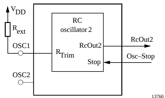
Figure 17. RC-oscillator 2
