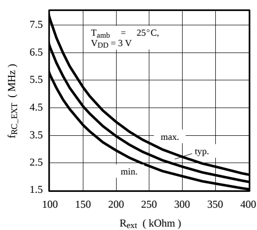
Figure 97. External RC frequency vs. R_{ext}
