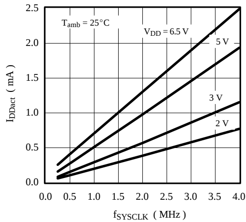
Figure 87. Active supply current vs. frequency
