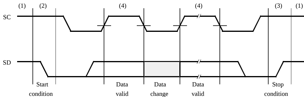
Figure 64. I 2 C bus protocol 1
