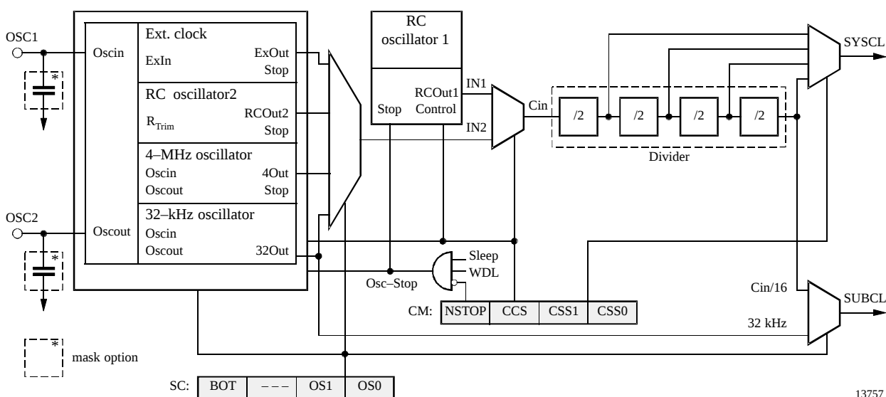
Figure 14. Clock module
