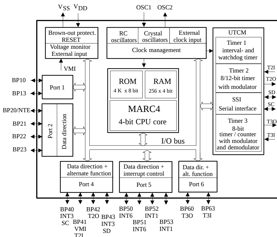
Figure 1. Block diagram M44C092-V
