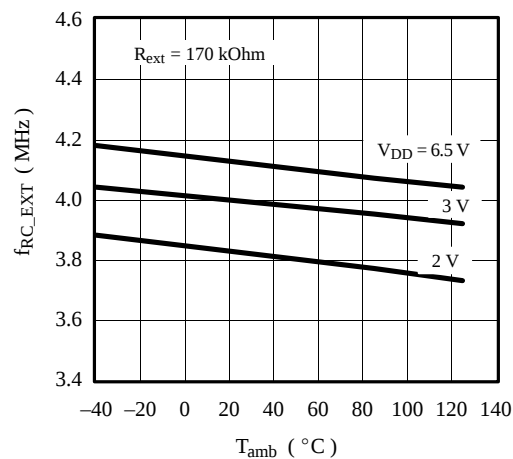
Figure 96. External RC frequency vs. T_{amb}
