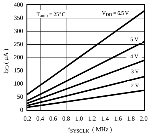
Figure 88. Power-down supply current vs. frequency
