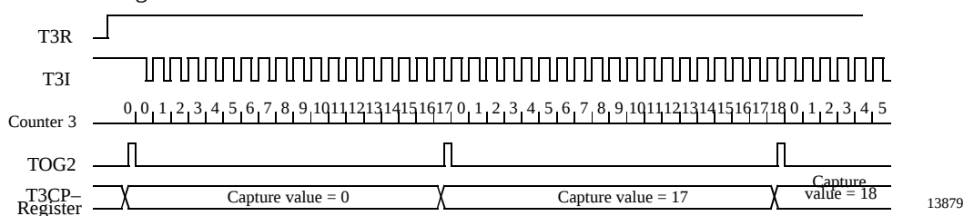
Figure 80. Frequency measurements
