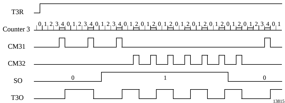
Figure 85. FSK modulation
