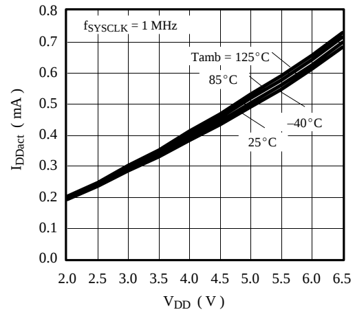
Figure 90. Active supply current vs. V_{DD}
