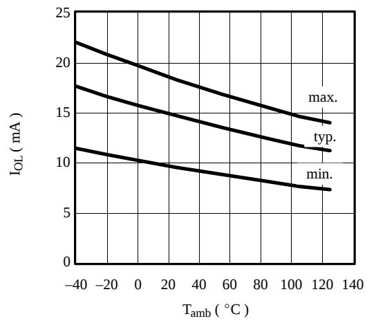
Figure 105. Output low current vs. T_{amb} V_{DD} = 6.5\text{ V} , V_{OL} = 0.2 \times V_{DD}
