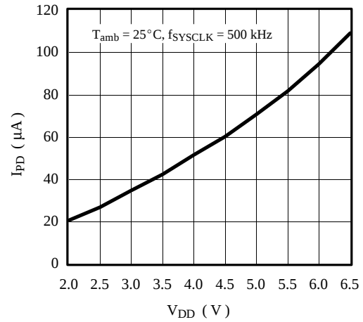
Figure 91. Power-down supply current vs. V_{DD}
