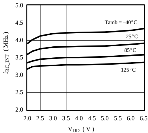
Figure 92. Internal RC frequency vs. V_{DD}
