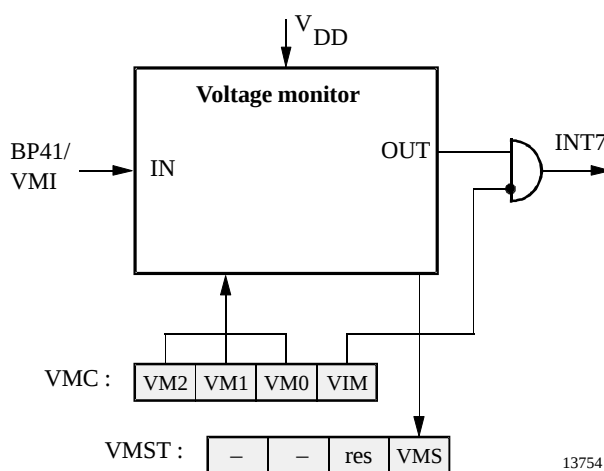
Figure 11. Voltage monitor
