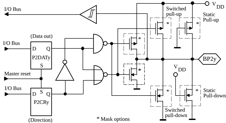
Figure 23. Bidirectional Port 2
