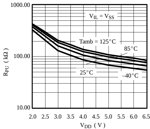
Figure 98. Pull-up resistor vs. V_{DD}
