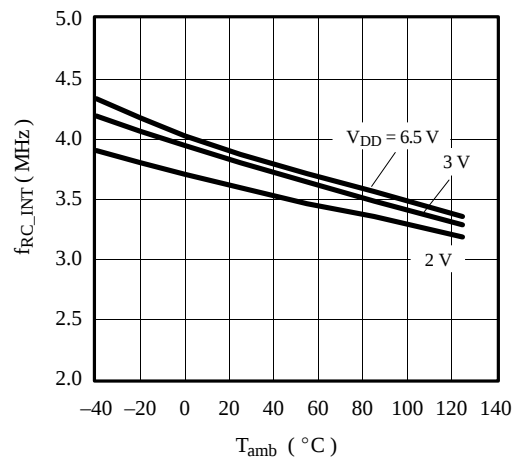
Figure 95. Internal RC frequency vs. T_{amb}
