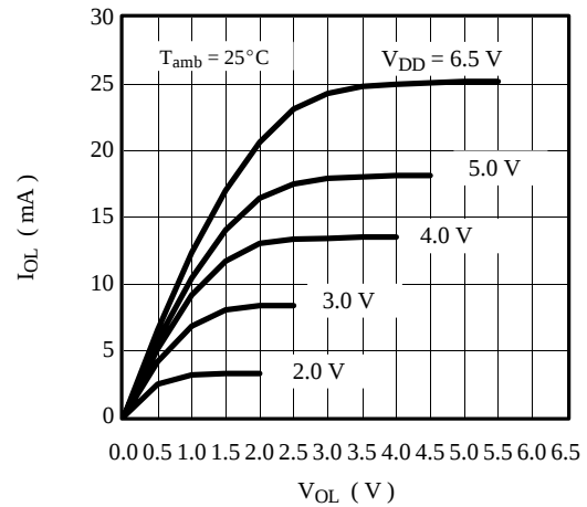
Figure 103. Output low current vs. output low voltage
