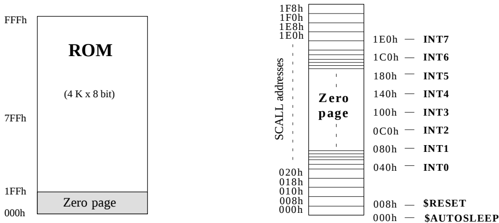
Figure 4. ROM map of M44C092-V
