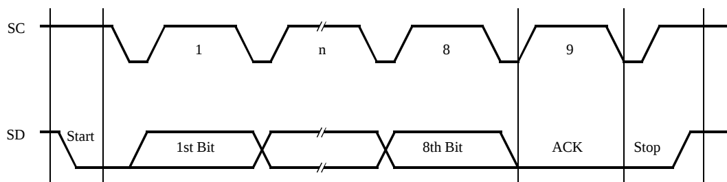
Figure 65. I 2 C bus protocol 2
