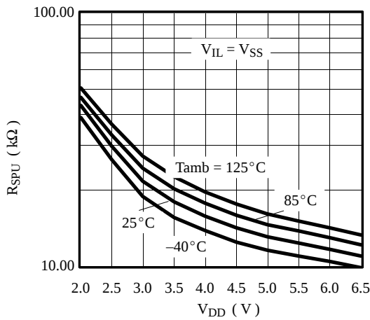
Figure 99. Strong pull-up resistor vs. V_{DD}
