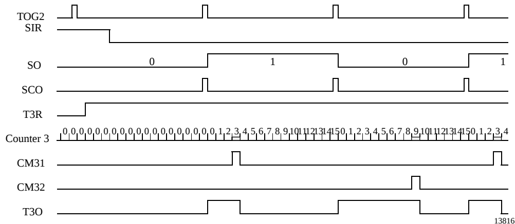
Figure 76. Pulse-width modulation
