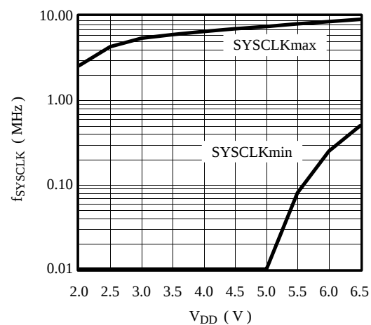
Figure 94. System clock vs. V_{DD}
