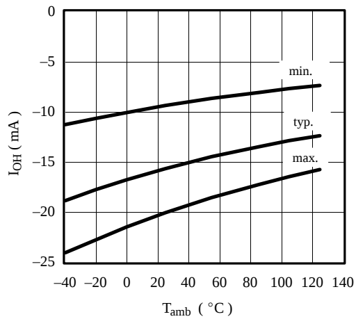
Figure 104. Output high current vs. V_{DD} = 6.5\text{ V} , V_{OH} = 0.8 \times V_{DD}
