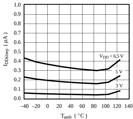
Figure 89. Sleep current vs. T_{amb}
