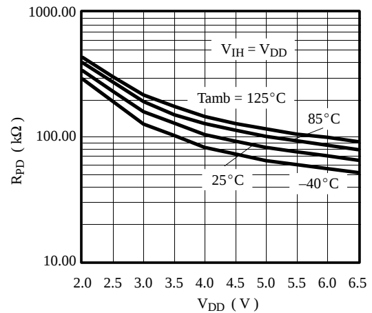
Figure 101. Pull-down resistor vs. V_{DD}
