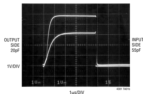
Input-Output Connection, t_{PHL}
