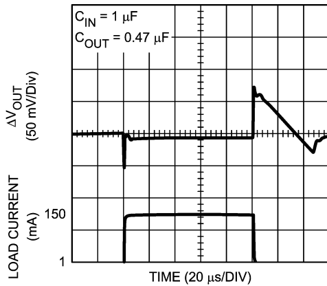
Load Transient
