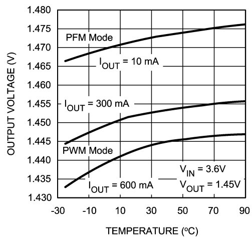
Output Voltage vs. Temperature, V_{OUT} = 1.45V
