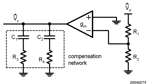
FIGURE 12. Compensation Network
