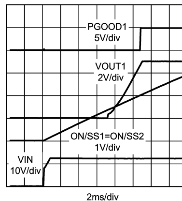
Power On and PGOOD1 Waveforms ( I_{OUT1} = I_{OUT2} = 0A )
