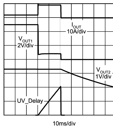
Over-Current and UVP Shutdown ( I_{OUT2} = 0A )
