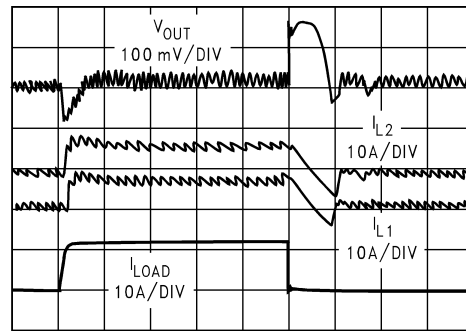
Load Transient Response Parallel Operation 1.8V OUT , 12V IN
