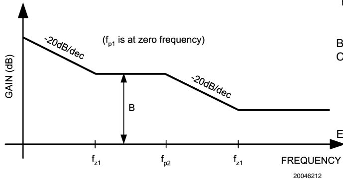
FIGURE 11. Output-Control Transfer Function
