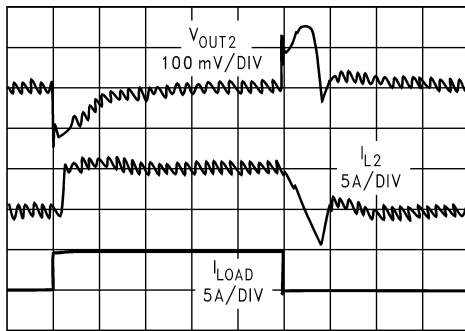
Ch.2 Load Transient Response 3.3V OUT , 12V IN
