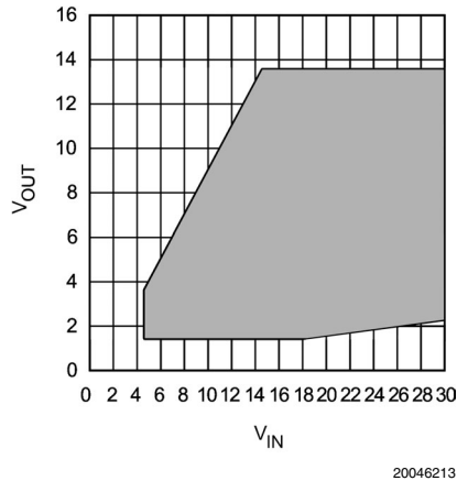
FIGURE 9. Output Voltage Range
