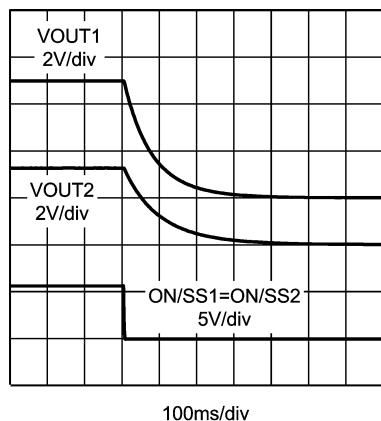
Shutdown Waveforms ( I_{OUT1} = I_{OUT2} = 0A )
