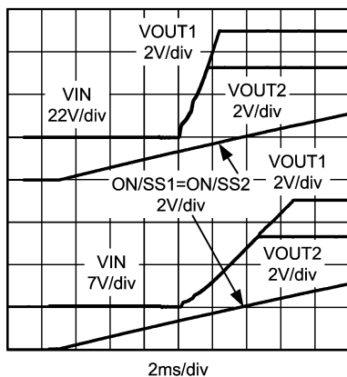
Softstart Waveforms ( I_{OUT1} = I_{OUT2} = 0A )
