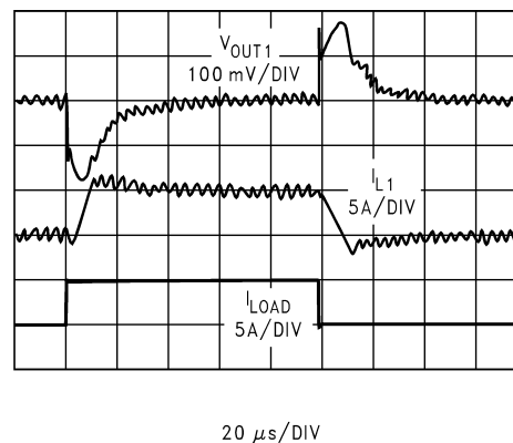
Ch.1 Load Transient Response 5V_{OUT}, 12V_{IN}
