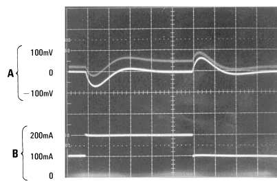
FIGURE 23. Line Regulation (Typical) of Flyback Regulator of Figure 22, +15V Output
