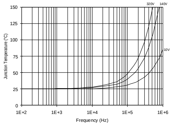
Figure 33. IR2113S T_J vs. Frequency (IRFBC30) R_{GATE} = 22\Omega , V_{CC} = 15V
