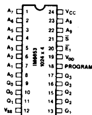
Figure 2: Pin Configurations
