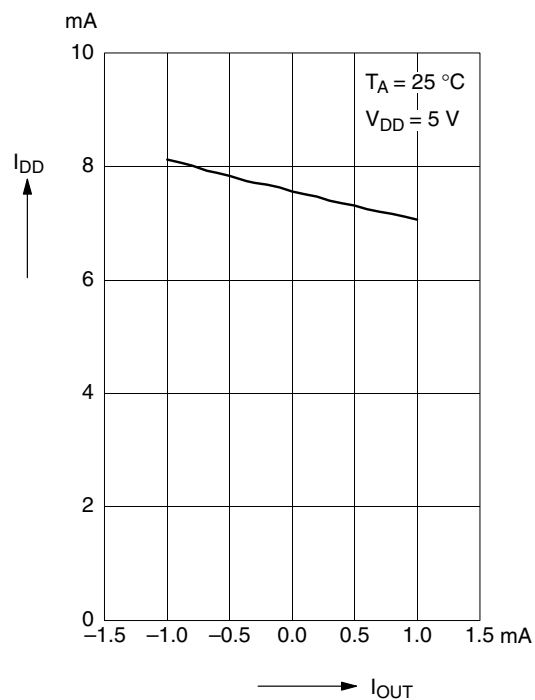
Fig. 3-7: Typical current consumption versus output current
