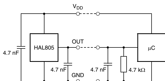
Fig. 4-1: Recommended application circuit
