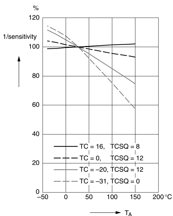
Fig. 3-10: Typical 1/sensitivity versus ambient temperature
