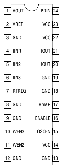
24-Pin QSOP
