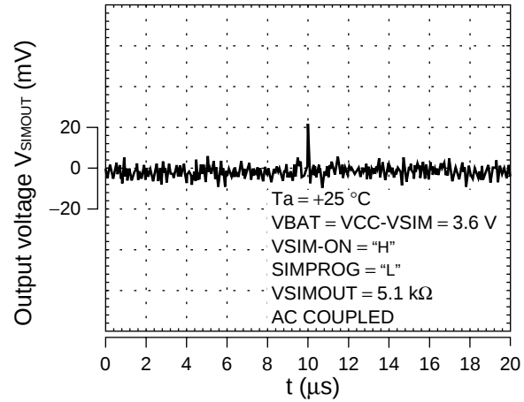
Output voltage waveforms (VSIMOUT Chargepump)
