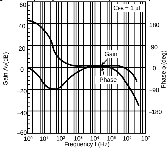
Fig. 19 - Frequency vs. Gain/Phase (Actual Data)
