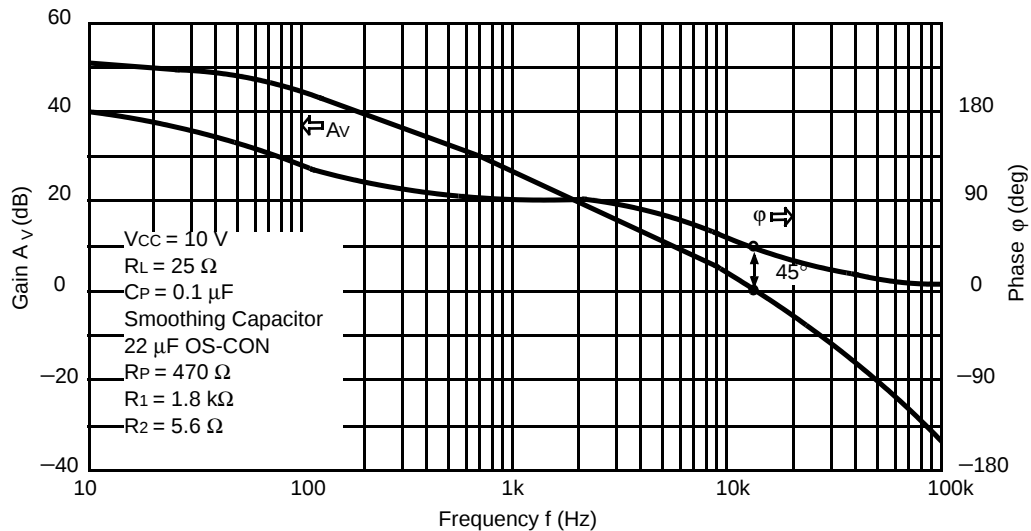
Fig. 38 - DC/DC Converter +5 V output
