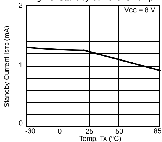
Fig. 25 -Standby Current vs.Temp.
