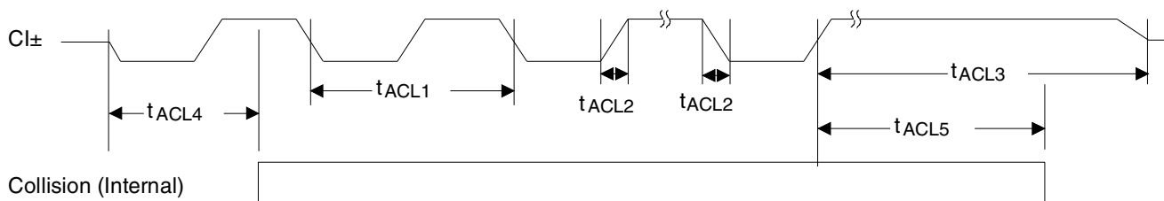
Figure 61. AUI Collision
