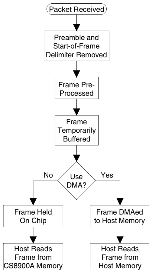
Figure 20. Frame Reception
