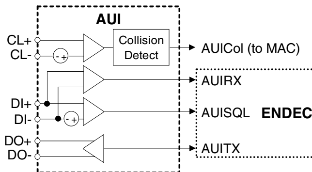
Figure 15. AUI
