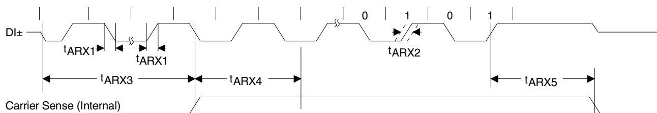
Figure 60. AUI Receive
