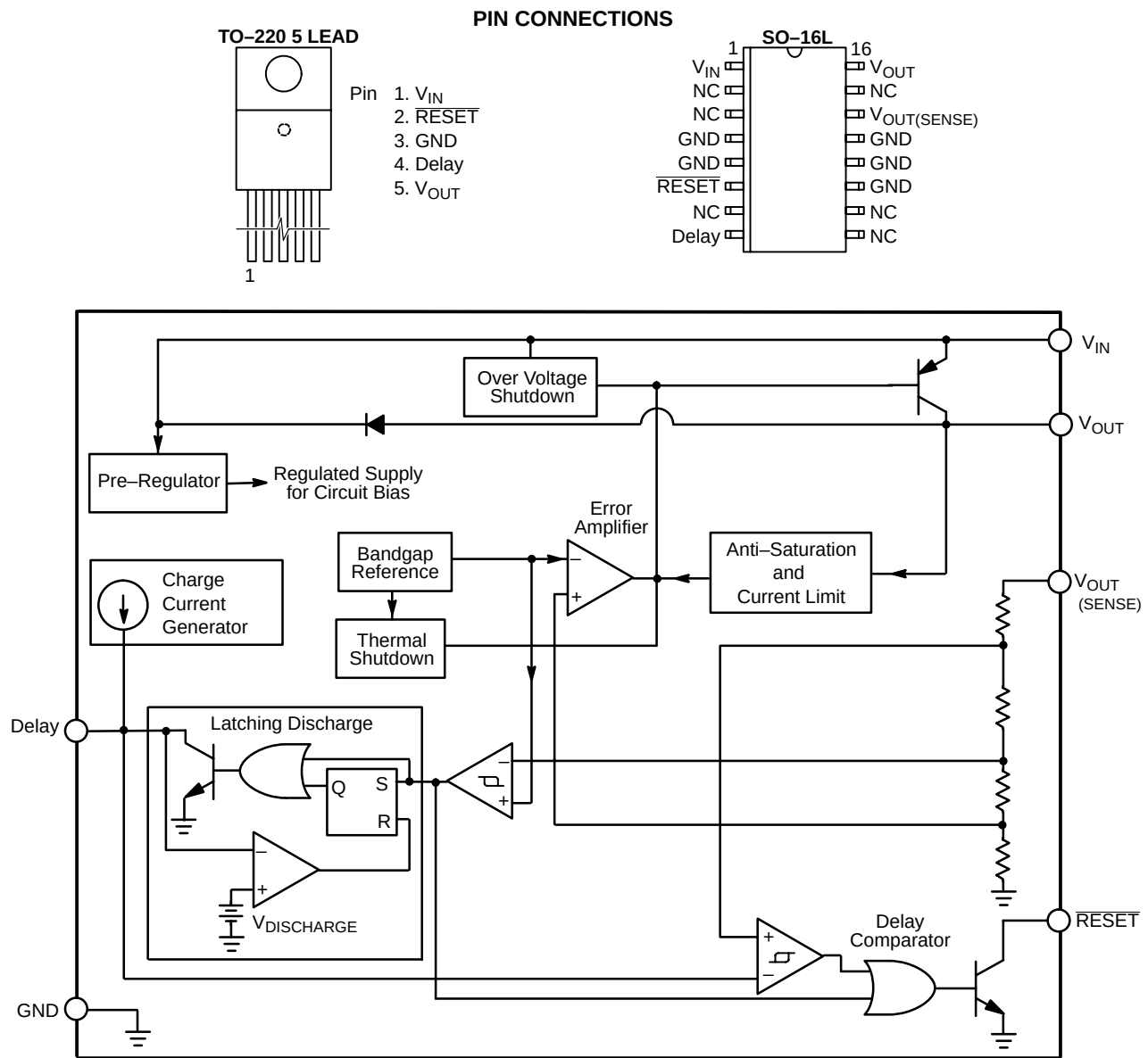
Figure 1. Block Diagram
