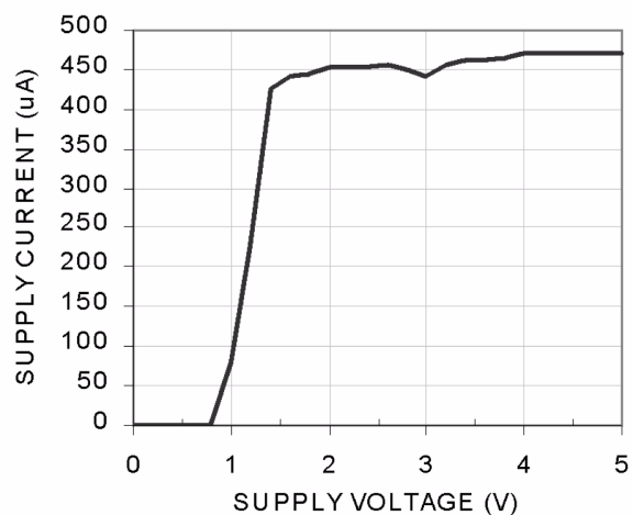
Figure 6. AV_{IN} Supply Current with Supply Voltage
