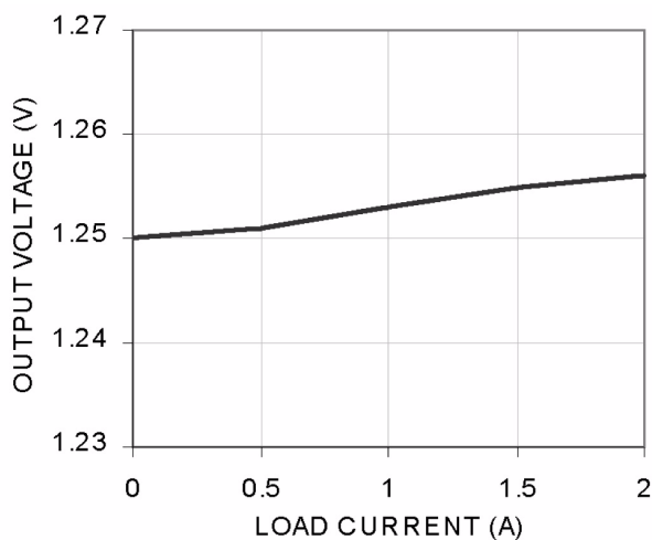
Figure 2. Load Regulation (Sink)
