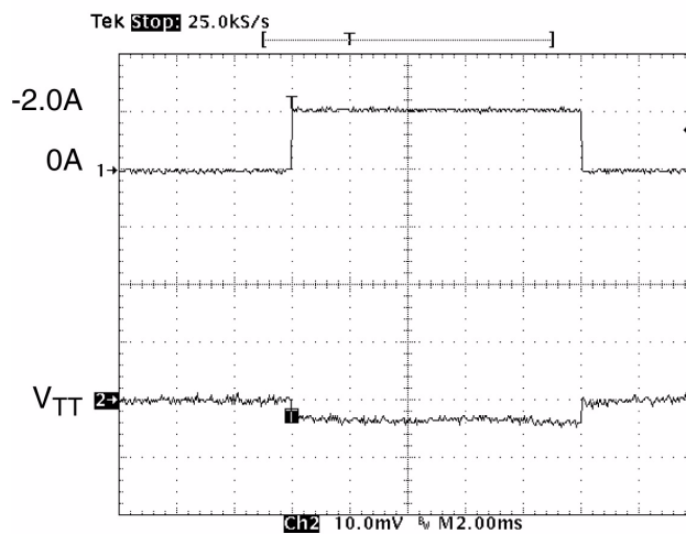
Figure 9. Line Transient (0A to 2.0A Source)
