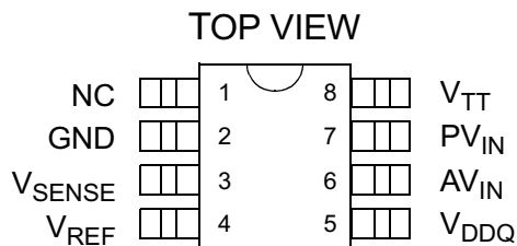
8-lead SOIC
