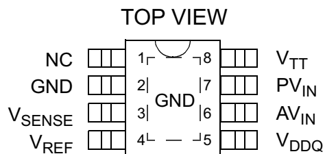
8-lead PSOP
