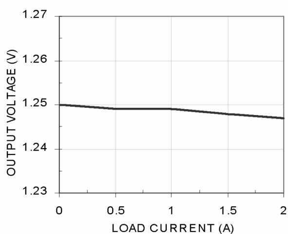
Figure 4. Load Regulation (Source)
