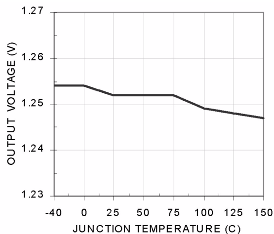
Figure 13. V_{TT} Output Voltage vs. Temperature (5mA load)
