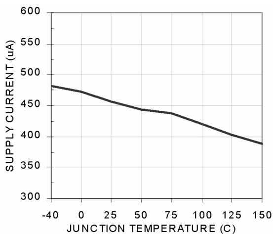
Figure 14. AV_{IN} Quiescent Current vs. Temperature
