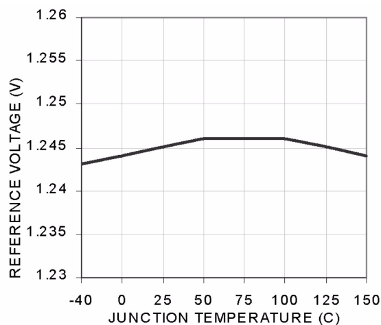
Figure 12. Reference Voltage vs. Temperature
