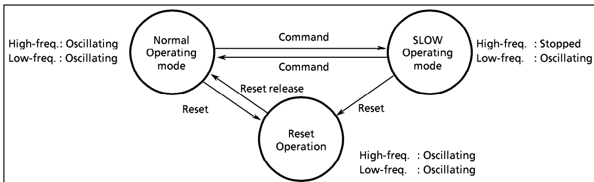
Figure 2-2. Operating Mode Transmission Diagram
