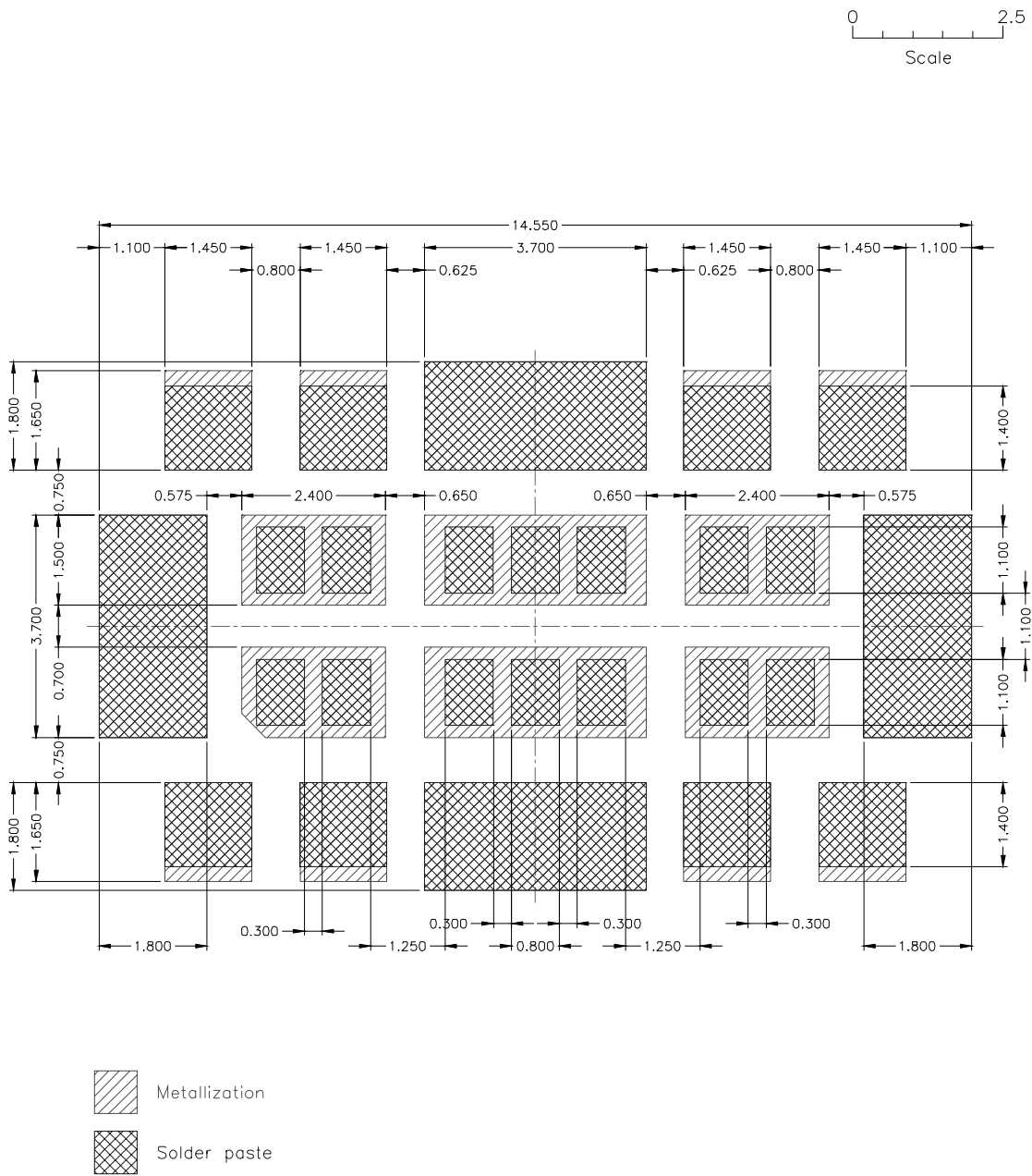
Fig.9 Soldering footprint for SOT632A.
