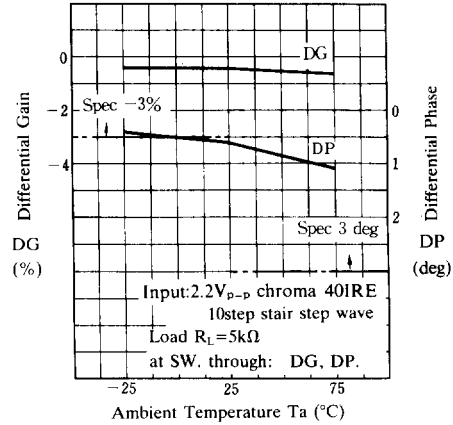
Differential Gain/Differential Phase ( V^+ = 5\text{V} )
