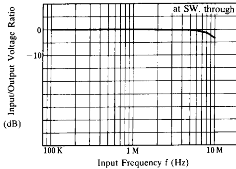
Video Switch Frequency Response ( V^+ = 5\text{V} , R_L = 5\text{k}\Omega , V_{IN} = 2V_{p-p} sine wave)
