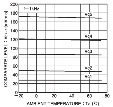
Fig. 7 Comparator level vs. ambient temperature
