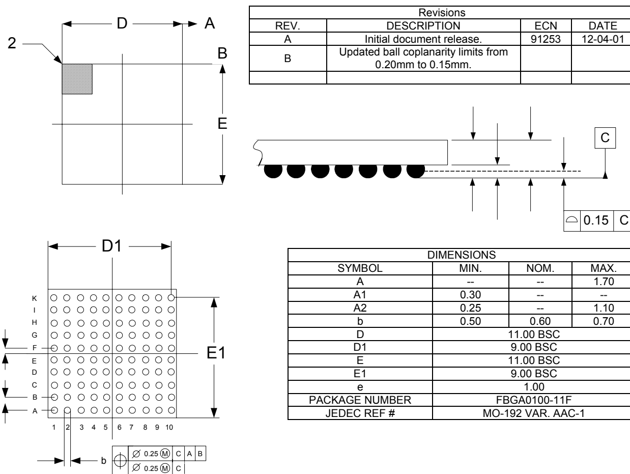
Figure 7 - FPBGA-100
