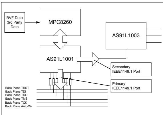
Figure 3 - Master mode
