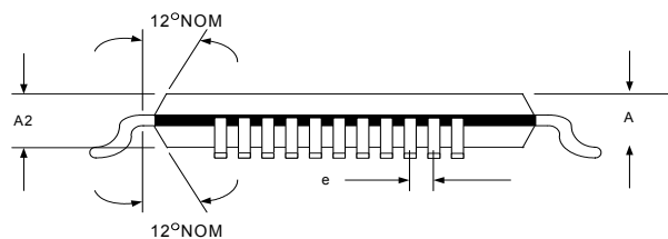
Figure 6 - LQFP-100
