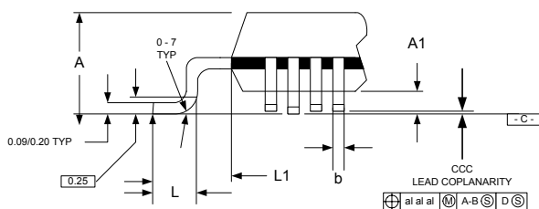
Figure 6 - LQFP-100
