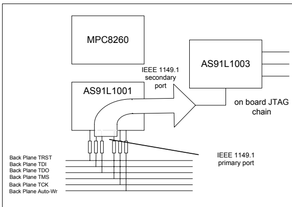
Figure 2 - Slave mode
