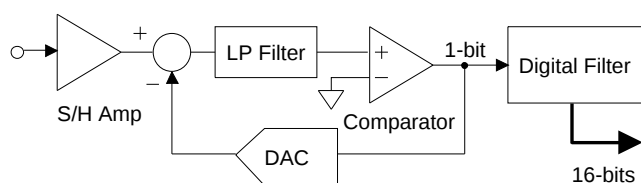
Figure 1. Delta-Sigma ADC
