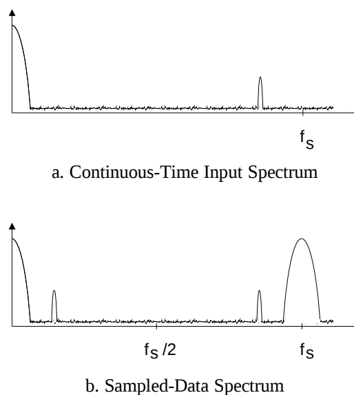
Figure 6. Sampled-Data Spectrum
