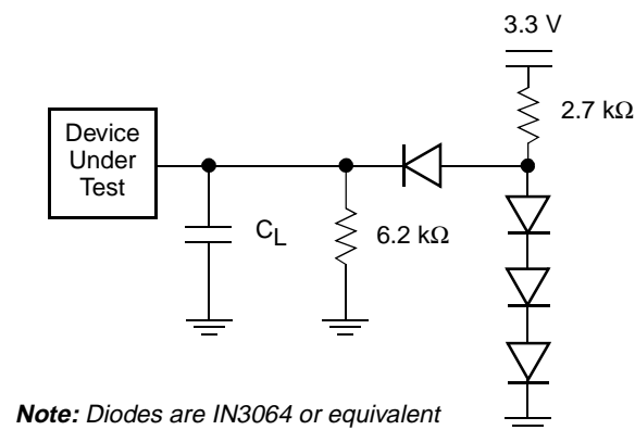
Figure 11. Test Setup
