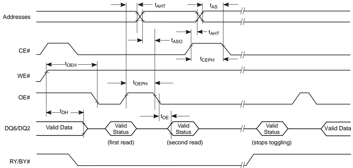
Figure 21. Toggle Bit Timings (During Embedded Algorithms)
