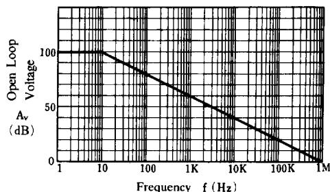
Open Loop Voltage Gain vs. Frequency
