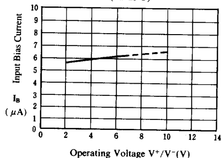
Input Bias Current vs. Operating Voltage
