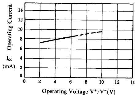
Operating Current vs. Operating Voltage
