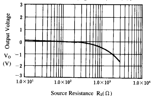
Output Voltage vs. Source Resistance
