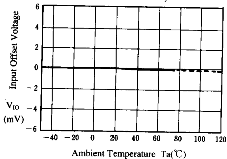
Input Offset Voltage vs. Temperature
