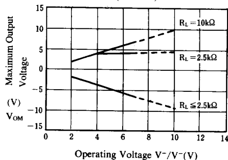
Maximum Output Voltage vs. Operating Voltage
