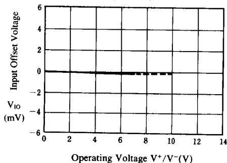
Input Offset Voltage vs. Operating Voltage
