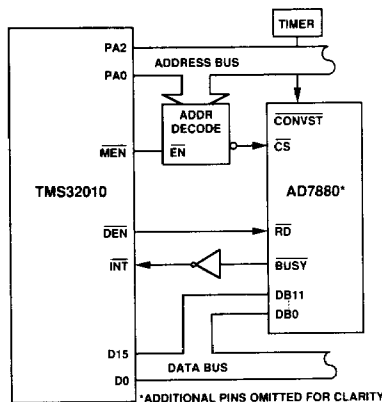
Figure 16. AD7880-TMS32010 Interface
