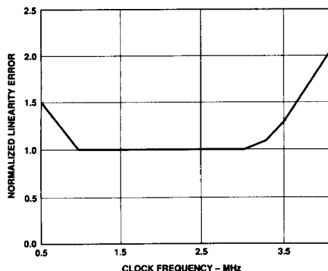
Figure 10. Normalized Linearity Error vs. Clock Frequency
