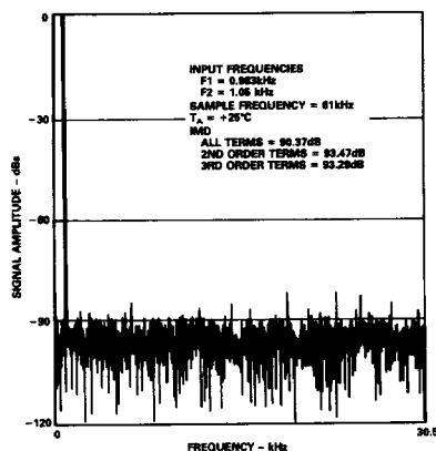
Figure 14. IMD Plot
