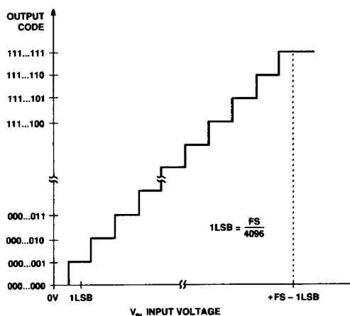
Figure 8. AD7880 Unipolar Transfer Characteristic
