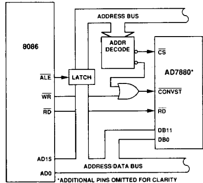
Figure 19. AD7880-8086 Interface
