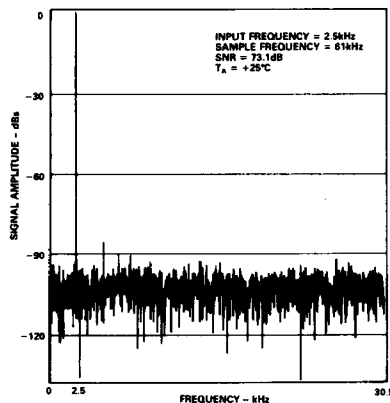
Figure 12. FFT Plot
