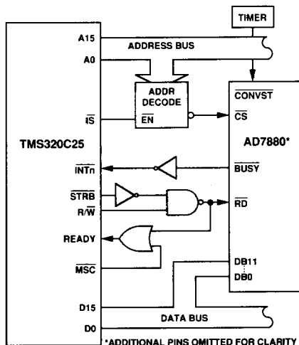
Figure 17. AD7880-TMS320C25 Interface
