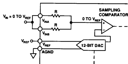
Figure 5. 0 to V_{REF} Unipolar Input Configuration
