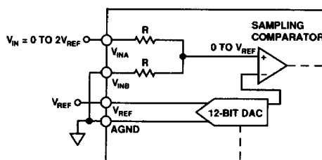
Figure 6. 0 to 2 V_{REF} Unipolar Input Configuration
