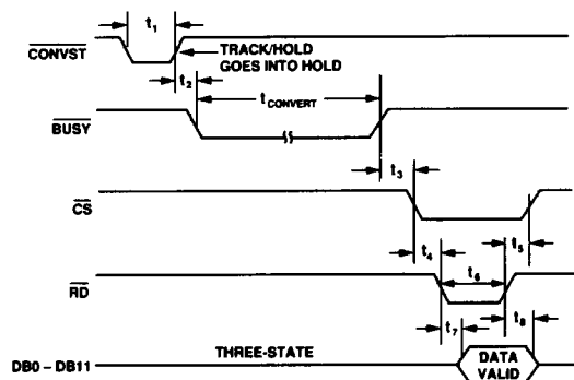
Figure 1. Timing Diagram
