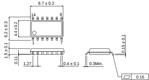
SOP14
