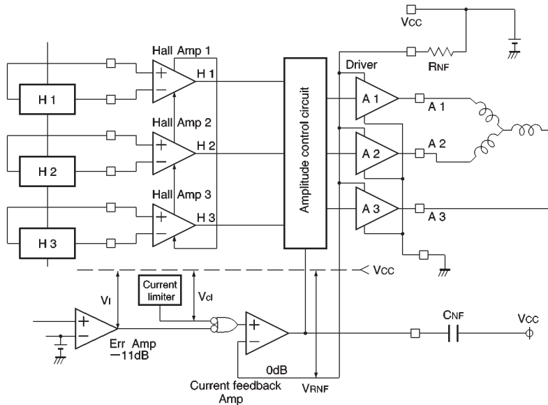
Fig.1 Motor drive circuit
