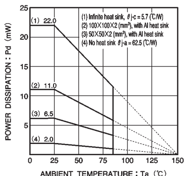
Fig. 6 Ta - power dissipation characteristics (TO220FP)
