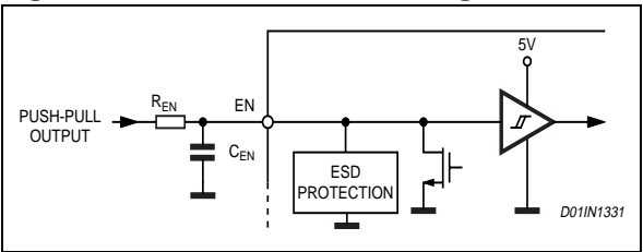
Figure 9. EN Pin Push-Pull Driving
