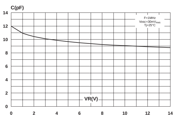
Fig. 2: Capacitance versus reverse applied voltage (typical values).
